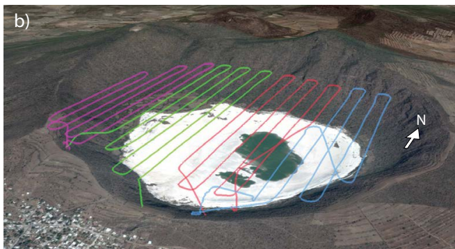
Figure 5. A total of 22 flight lines were required to cover the crater's 1.2 km x 1.2 km bottom. The flight lines shown were registered by the GPS watch attached to the quadcopter and visualized on Google Earth: (a) plan view, where the distance between flight lines can clearly be seen, and (b) perspective view showing both take-off and landing points as well as the elevation of all flight lines; flight elevations were set at 1900 m a.s.l. The turns at the end of each flight line were set as adaptive bank turns and a total of four flights were required; the quadcopter was landed at the end of each flight to replace the battery.
