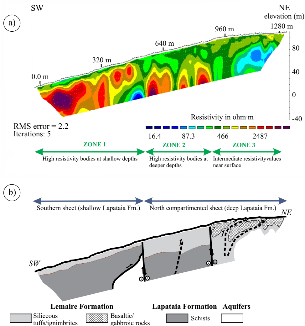
Figure 6. a) Electric resistivity tomography (ERT) section (location in Figure 3) and b) geological interpretation.
