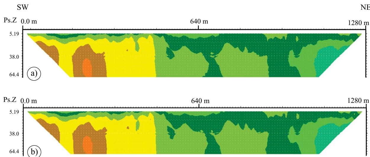
Figure 5. a) Apparent resistivity pseudosection from field measurements (see Figure 3 for location). Wenner-Schlumberger array, unit electrode spacing of 10 m. b) Calculated apparent resistivity pseudosection.
