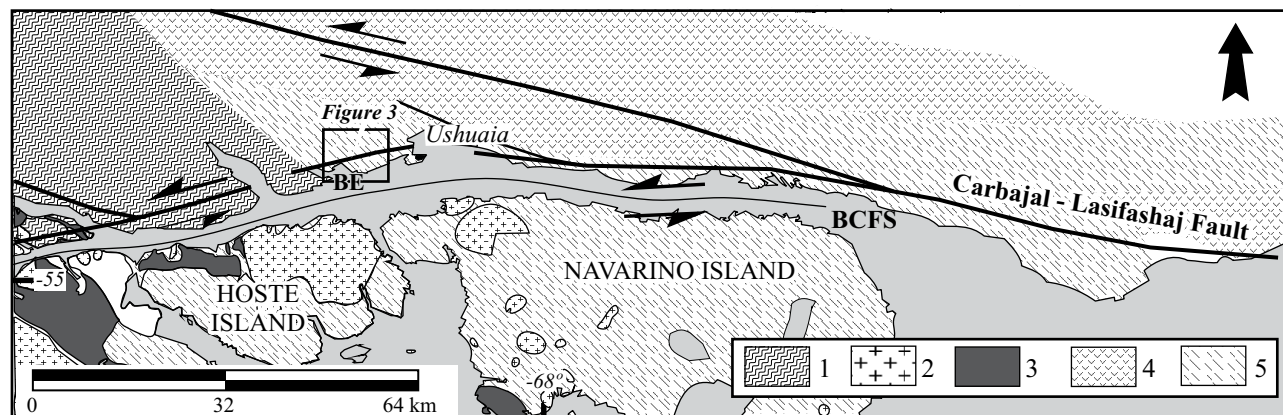
Figure 2. Simplified geological map of the Beagle Channel area. 1: Lapataia Fm.; 2: intrusive bodies of the Fuegian Batholith; 3: Tortuga Complex (basaltic/gabbroic rocks); 4: Lemaire Formation; 5: Yahgán Formation. BCFS: Beagle Channel Fault System; BE: Bahía Ensenada.
