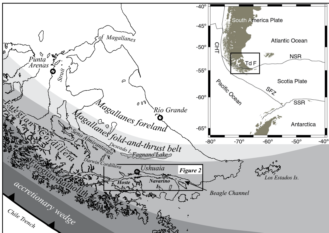
Figure 1. Major morphotectonic provinces in the region of Tierra del Fuego. Inset shows main plates and plate boundaries in the South Atlantic. TdF: Tierra del Fuego; NSR: North Scotia Ridge; SSR: South Scotia Ridge; SFZ: Shackleton Fracture Zone; CHT: Chile Trench.
