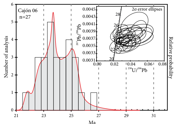
Figure 9. Probability density function and histogram of U/Pb ages from sample Cajón 06 (21.42845°N; 104.57444°W). Upper right insert shows U/Pb Concordia diagram of analyzed grains. Analytical data are provided in Supplemental file 2.
