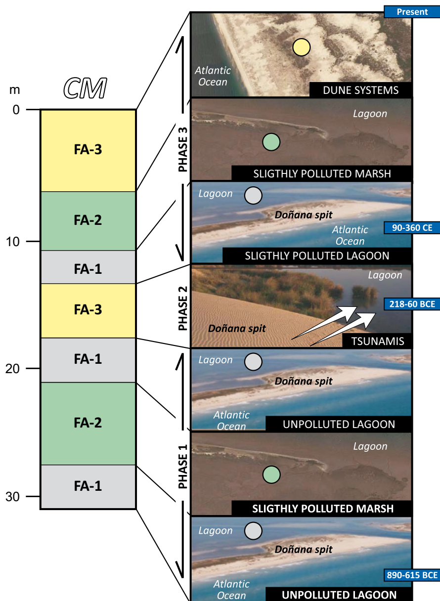
Figure 4. Paleoenvironmental evolution of core CM.
