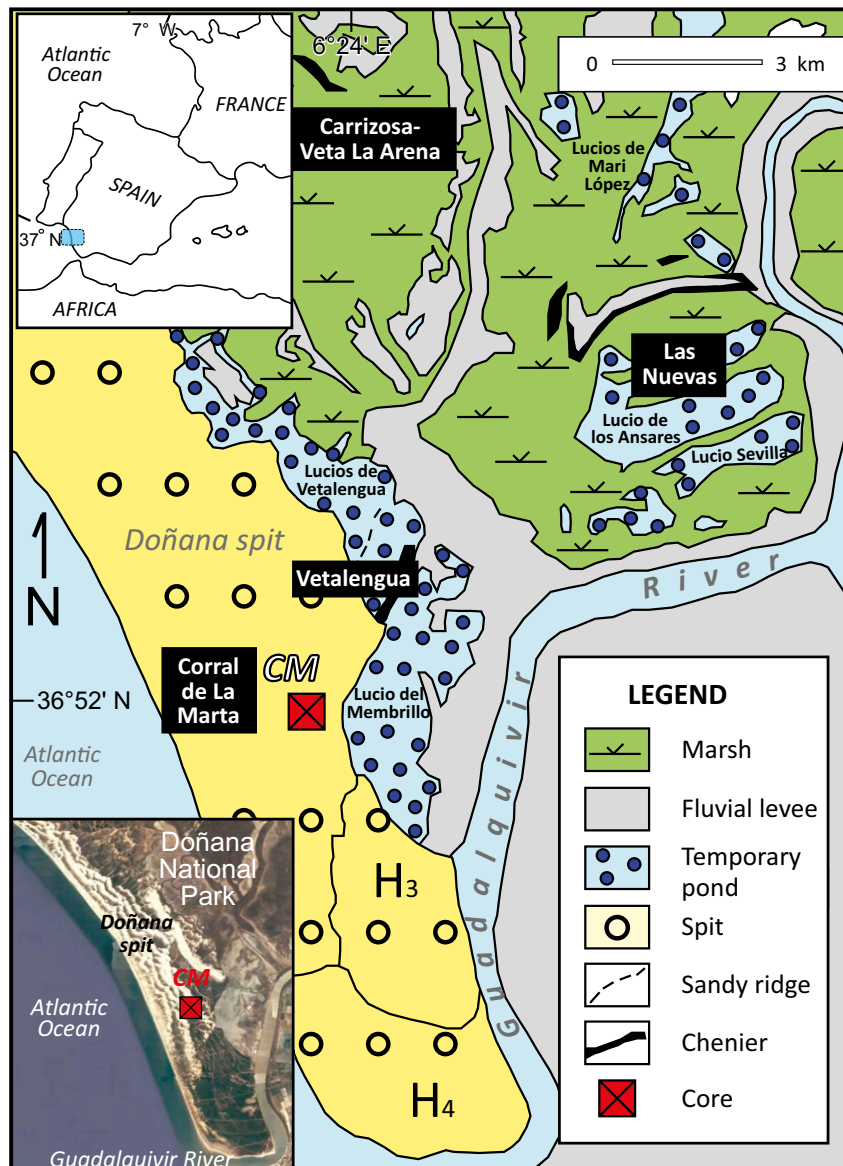
Figure 1. Main geomorphological features of the Doñana National Park, with location of the core studied. H3-H4: progradation phases (see text).
