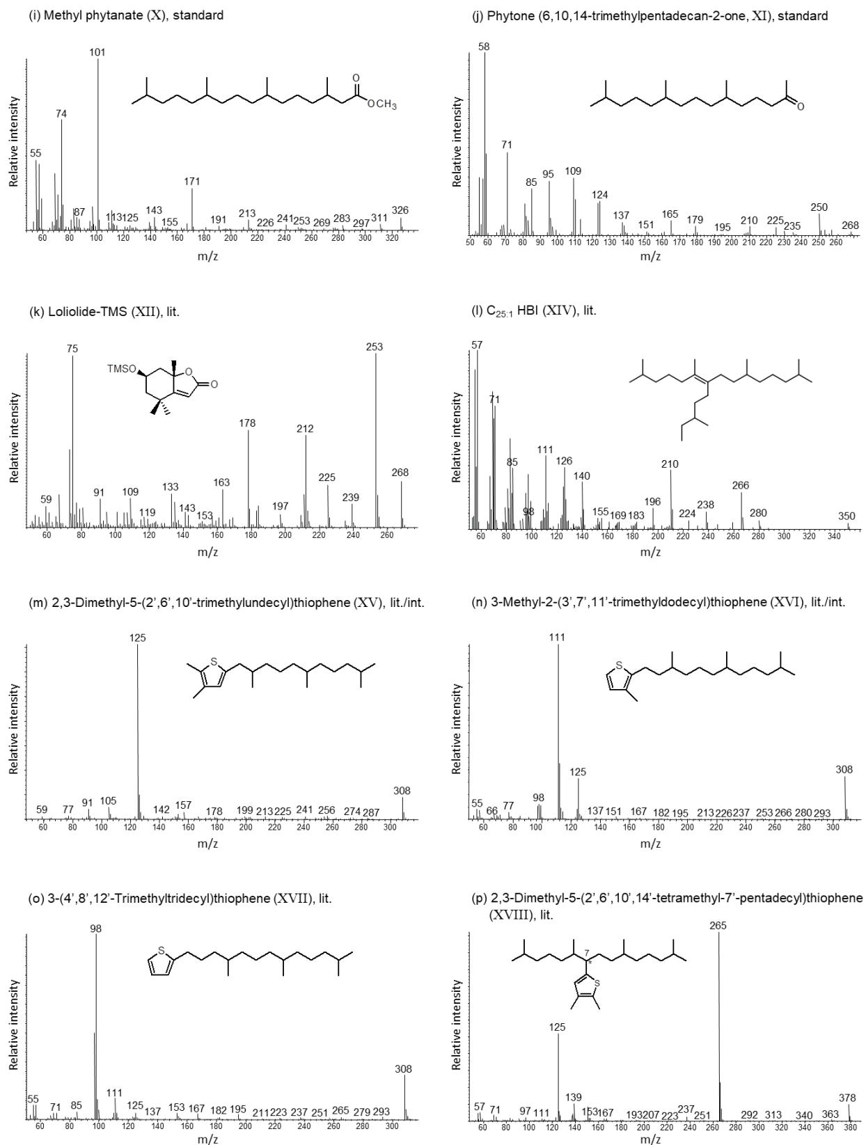
Figure SM2 (cont.). Mass spectra of compounds identified in this study. Note: lit. = mass spectrometric data published in the literature; int. = interpretation of mass spectrometric fragmentation pattern with respect to related compounds.
