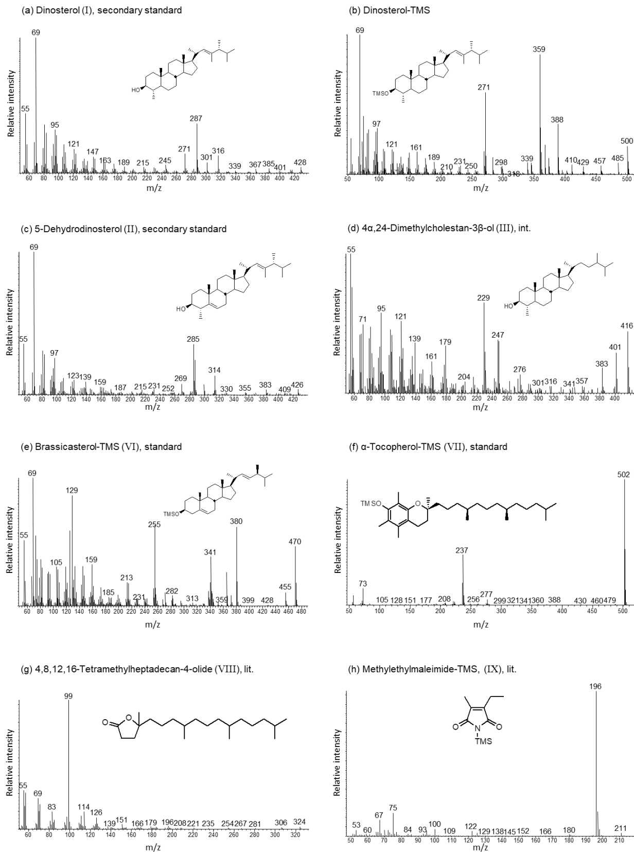
Figure SM2. Mass spectra of compounds identified in this study. Note: lit. = mass spectrometric data published in the literature; int. = interpretation of mass spectrometric fragmentation pattern with respect to related compounds.
