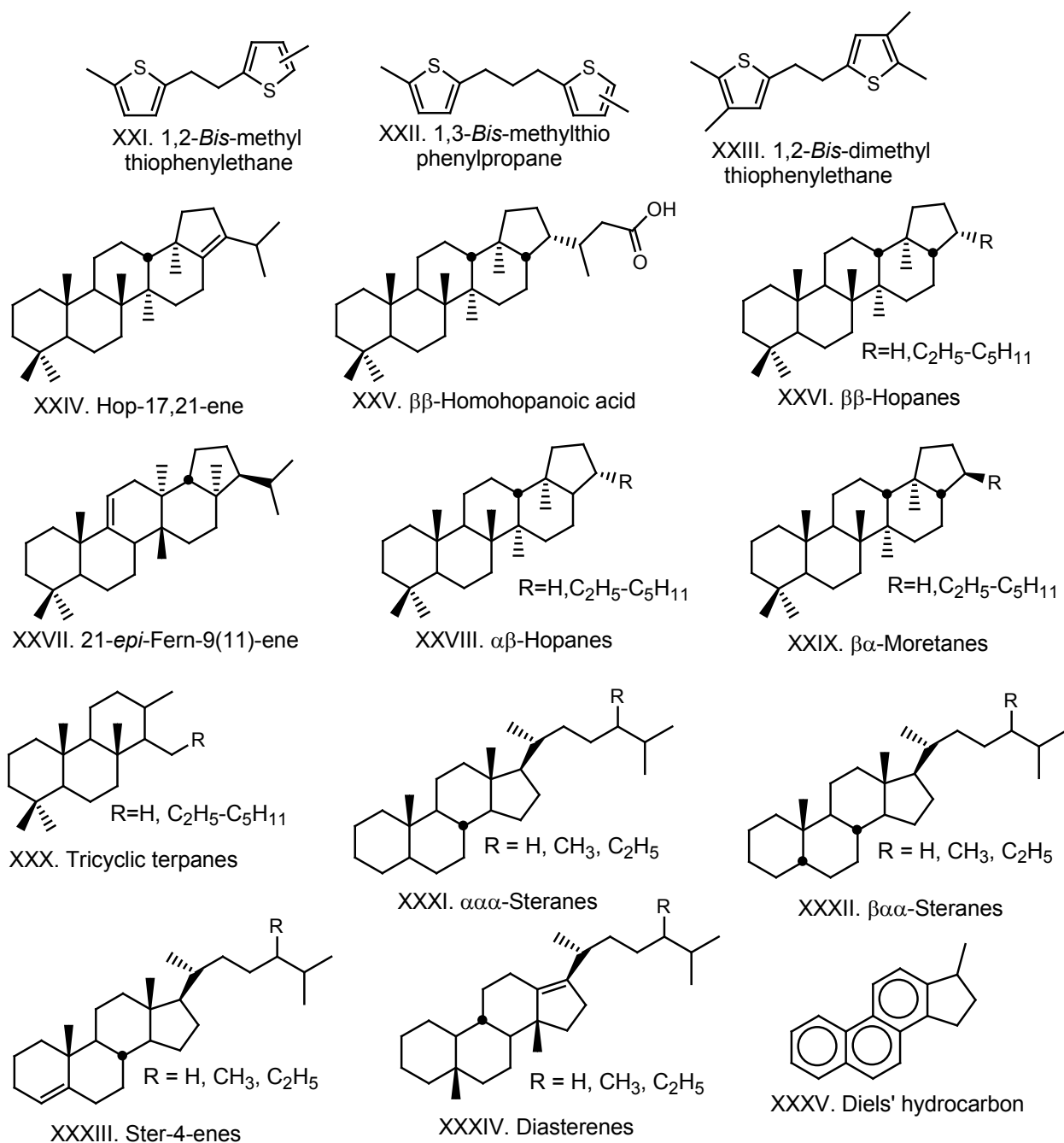
Appendix SM1 (cont.). Chemical structures cited.
