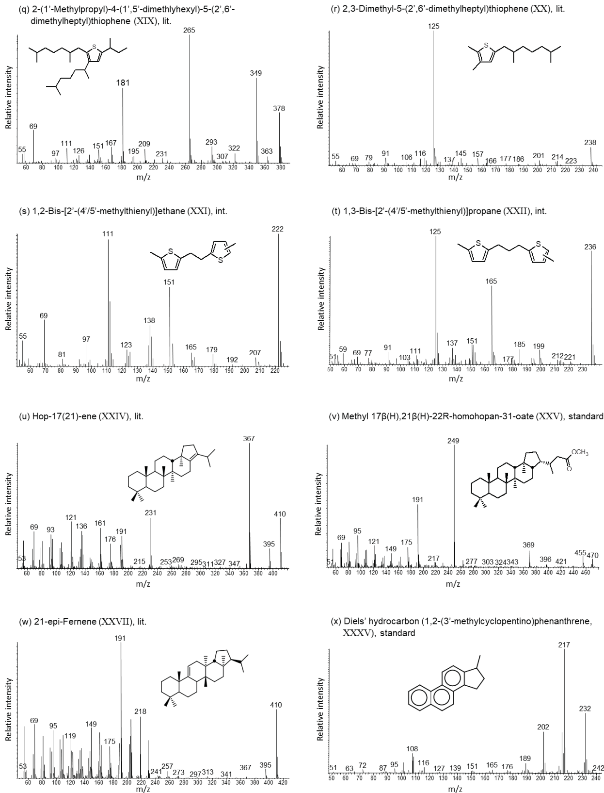
Figure SM2 (cont.). Mass spectra of compounds identified in this study. Note: lit. = mass spectrometric data published in the literature; int. = interpretation of mass spectrometric fragmentation pattern with respect to related compounds.
